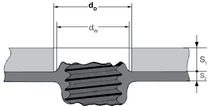
Clearance hole d_b for clamped material d_w : bulge diameter d_b : clearance hole
