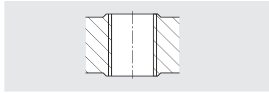
Screw installation without countersink (small bulge)
