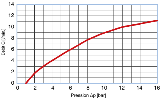
CHECK VALVE® Courbe de flux – unscreened BF660080024100; T = 50 °C, huile hydraulique HLP46
