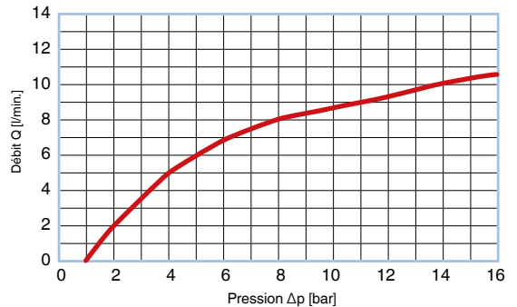
CHECK VALVE® Courbe de flux – screened BR660080024100; T = 50 °C, huile hydraulique HLP46
