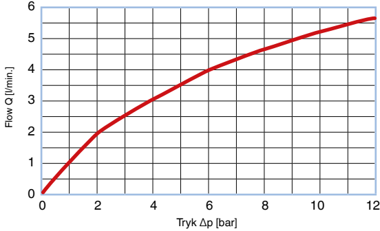
CHECK VALVE® Flowkurve – unscreened BFAA055U014; T = 50 °C, hydraulikolie HLP46
