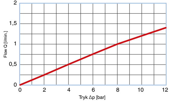
CHECK VALVE® Flowkurve – screened BFAA055014; T = 50 °C, hydraulikolie HLP46
