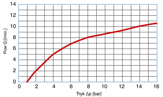
CHECK VALVE® Flowkurve – screened BR660080024100; T = 50 °C, hydraulikolie HLP46
