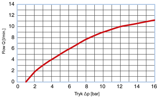
CHECK VALVE® Flowkurve – unscreened BF660080024100; T = 50 °C, hydraulikolie HLP46
