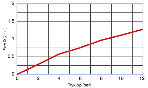
CHECK VALVE® Flowkurve – screened BFAA055014; T = 50 °C, hydraulikolie HLP46
